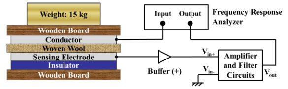
Figure 3. Experimental setup for measuring frequency-gain characteristics.
